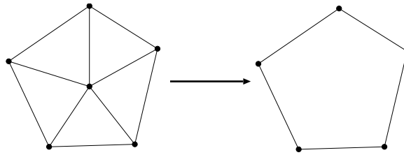
図 7.8: removeVertexInLoop
