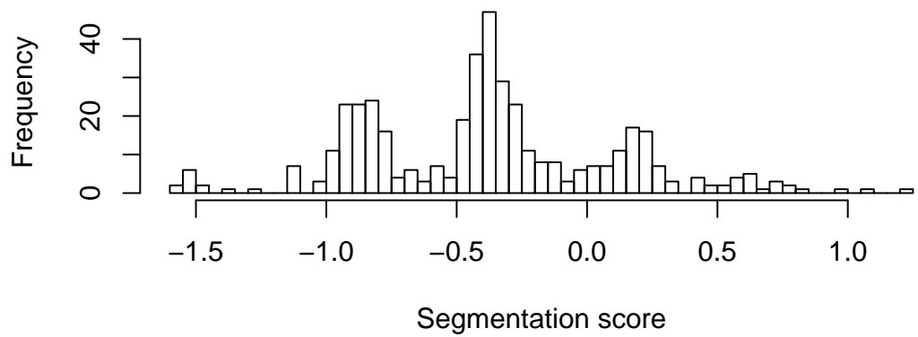
Figure 7: Clustering results of European-ancestry sample sets.
