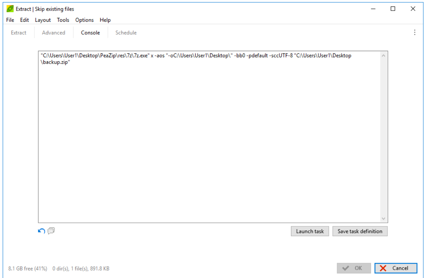
Image 17: Console tab
